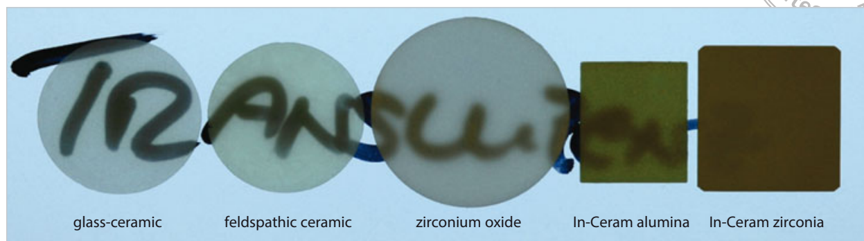
Fig 1a Translucency of 0.5-mm-thick plates of different materials: glass-ceramic, feldspathic ceramic, zirconium oxide, In-Ceram alumina, and In-Ceram zirconia.
